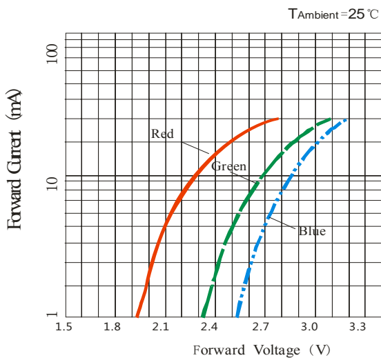
Volt-Ampere Characteristics
