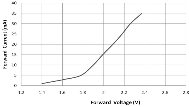
Forward Current VS. Forward Voltag (Ta=25°C)
