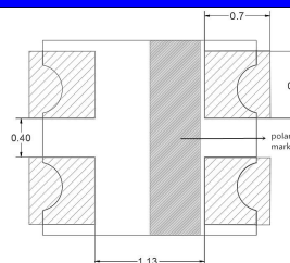
PCB Solder Pad
